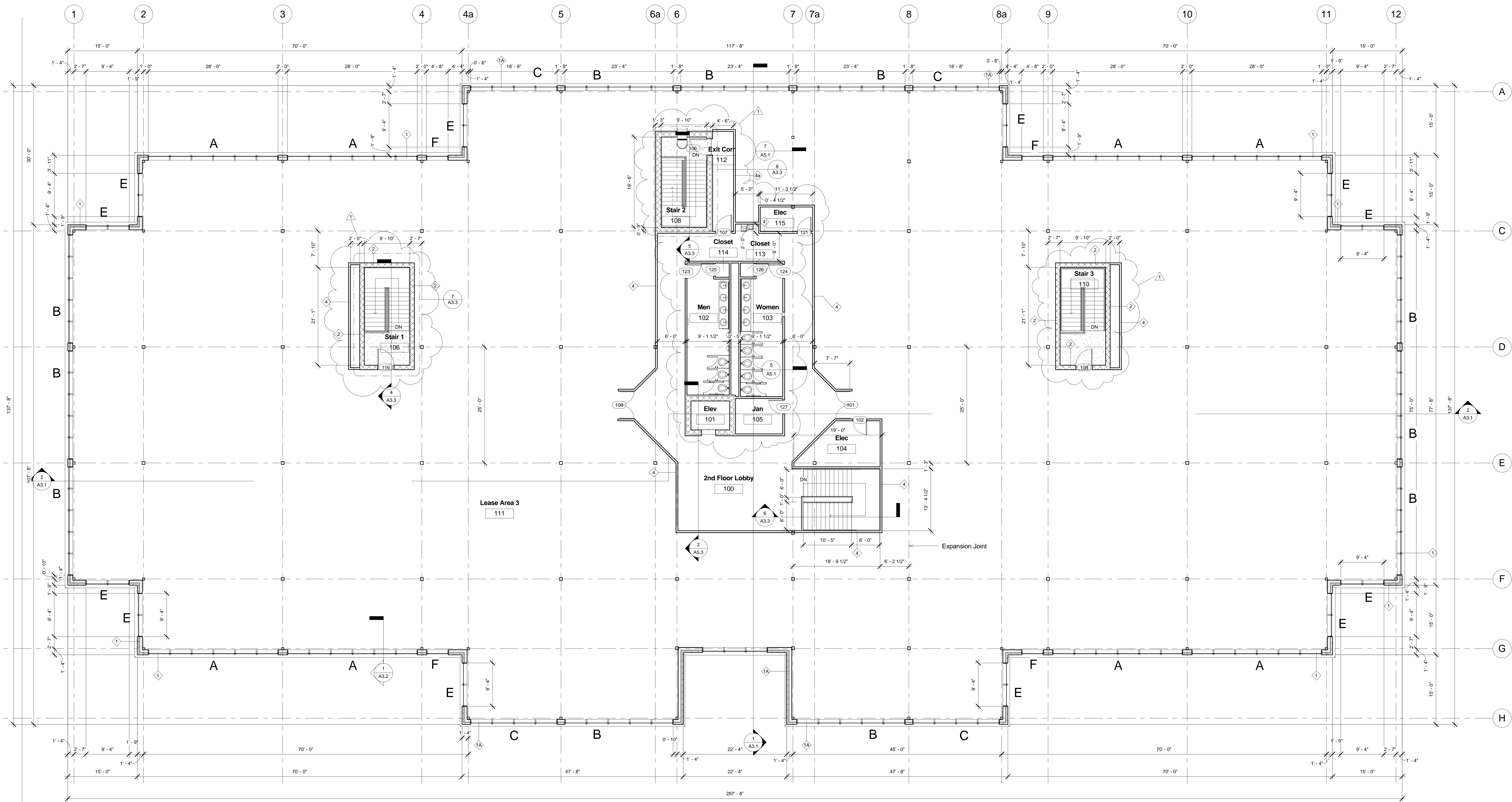
1 Second Floor Plan 1/8" = 1'-0"
