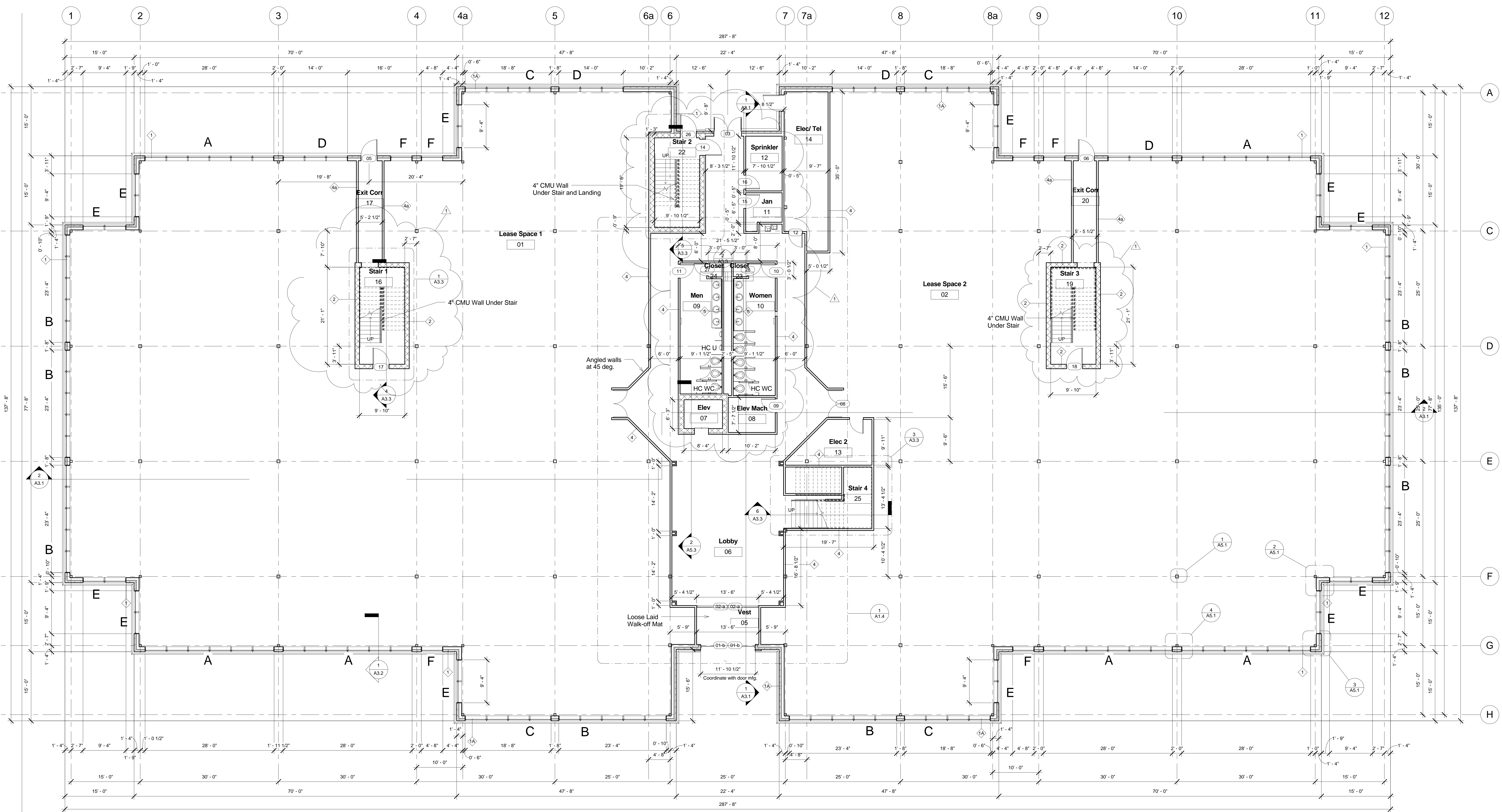
1 First Floor Plan 1/8" = 1'-0"
